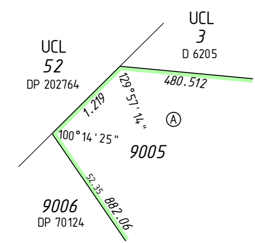
ENLARGEMENT 'E1' Not to scale
